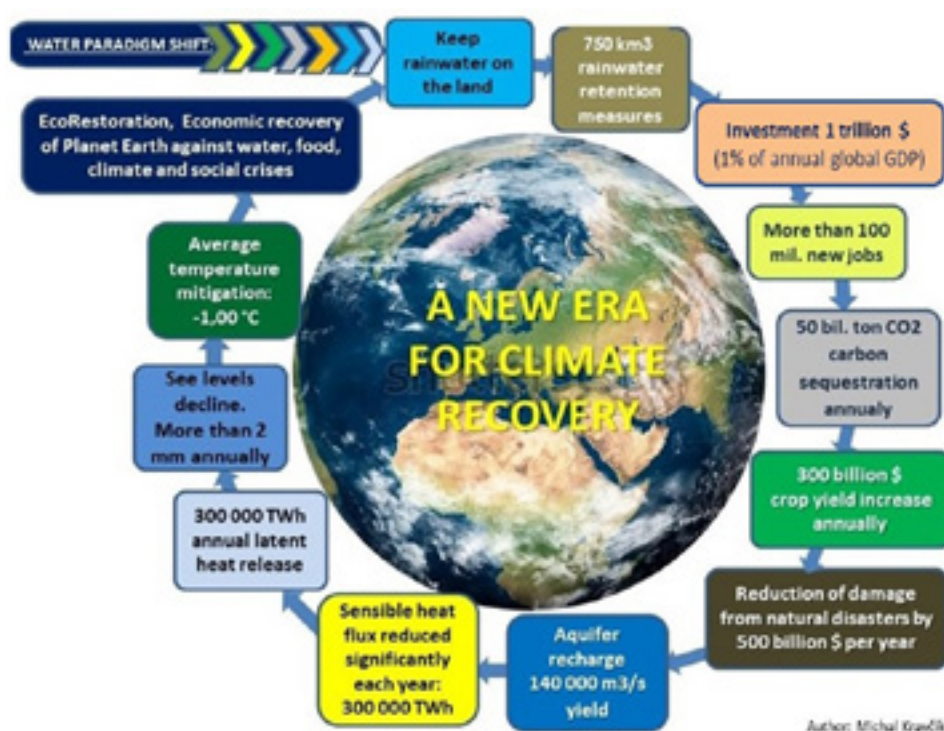
Scheme 1: New Water Paradigm shift provides global system solutions. Keeping rainwater on the land will renew small water cycle flow and moisture recycling, augment water resources, increase carbon sequestration, decrease temperatures, create new jobs, and mitigate climate risks, such as floods, droughts, and sea level rise.
